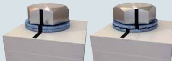
When untightening a bolt secured by Nord-Lock washers, check that sliding occurs between the cam faces.
